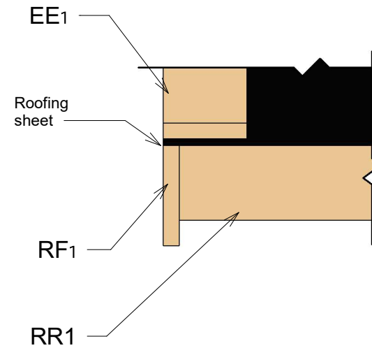
3 Roof Reinforcement
