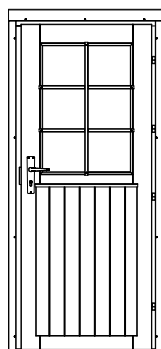
Single Door db. gl 2 st. 70 mm L+R 840 x 1955 mm +12 mm
